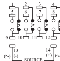
H3Y-4 (FOUR SET CONTACT)
