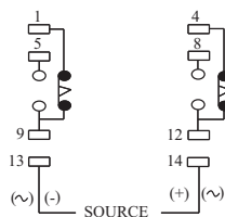
H3Y-2 (DOUBLE CONTACT)
