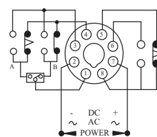
AH2-N/Y,H3M,H3CT (A/B CONTACT)
