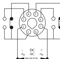
AH3-3 (TIME DELAY + INSTANT CONTACT)
