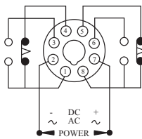
AH3-2 (DOUBLE CONTACT)
