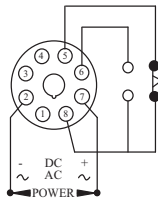
AH3-1 (SINGLE CONTACT)
